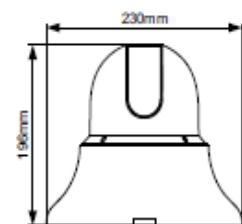
Surface Mount
