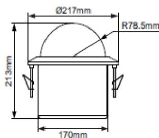
In-Ceiling Mount
