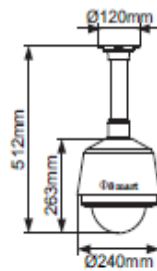
Pole Mount
