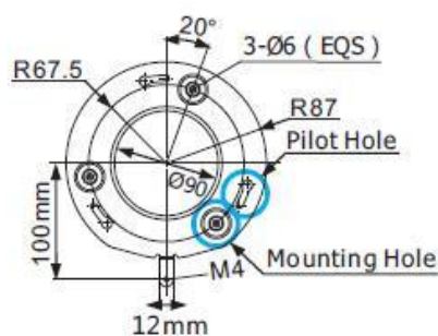
Mounting Plate
